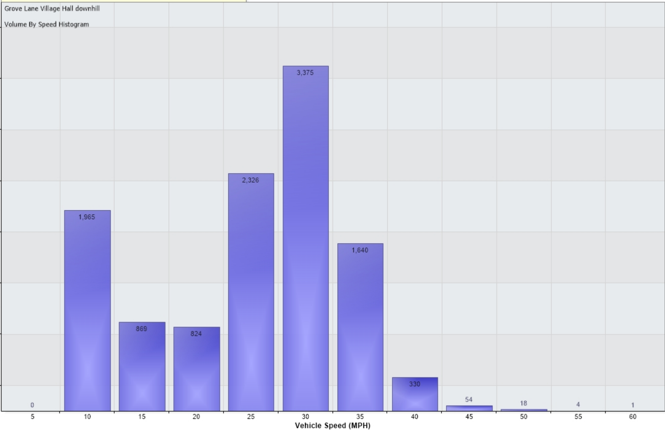
Vehicle Counts Vs. Speed [Grove Lane Village Hall downhill: Incoming]
